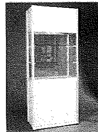
FA017 Tall Showcase - 2 Layers of Glass Shelf, 2 x 50 Watt Halogen Downlights (Yellow Light) (1mL x 0.5mD x 2.5mH) 高身陳列飾櫃連兩層玻璃層板及兩盞50瓦特 鹵素射燈 (黃光) (1米闊 x 0.5米深 x 2.5米高)
